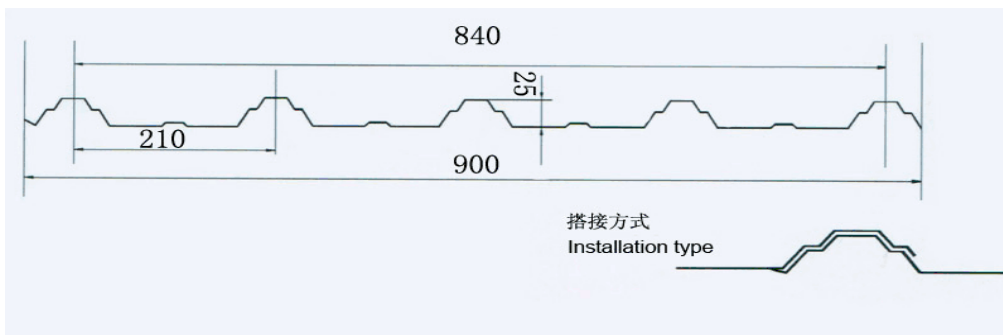
Pic.1 V25-210-840 Aluminium Corrugated Sheet
