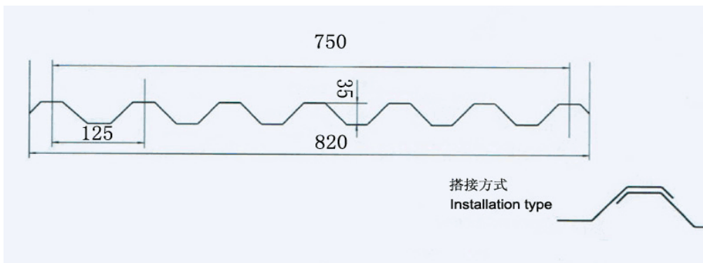
Pic.2 V35-125-750 Aluminium Corrugated Sheet
